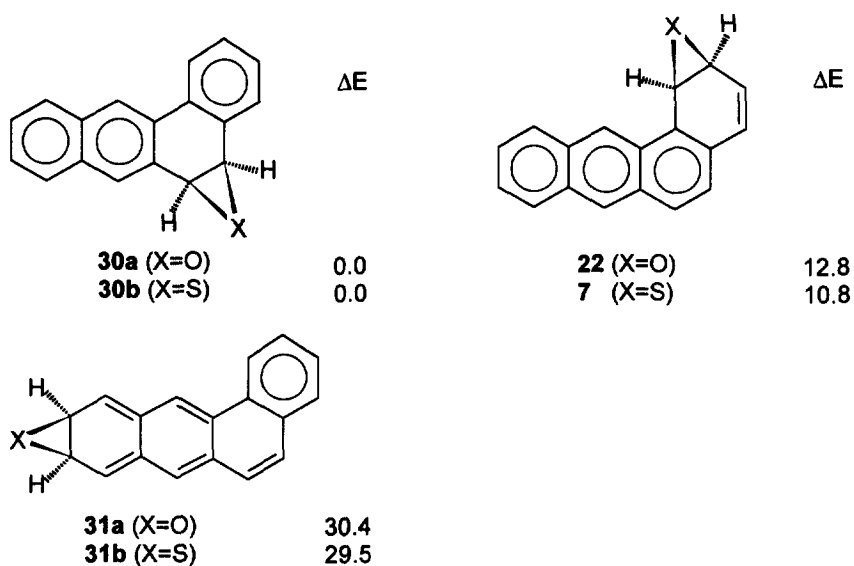
Scheme 2. Relative energies (kcal/mol) of benz[a]anthracene oxides and episulfides.
